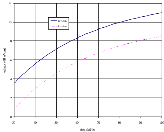
Figure 6. E_{\max}^d for 3 m and 4 m separation distance for a horizontally-polarized antenna. The transmit antenna height is 1 m, and the receive antenna height is scanned from 1 to 4 m.
