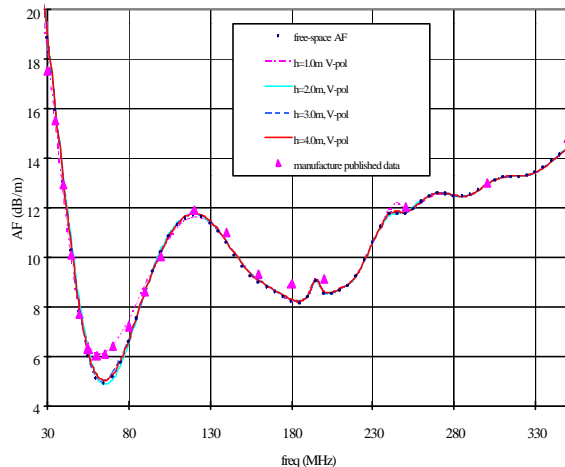
Figure 4. Numerically-calculated bicon/log hybrid AF at different heights for vertical polarization above a conducting ground plane. Manufacturer-published data are also shown as triangles.
