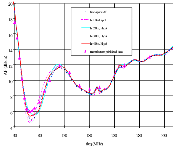
Figure 3. Numerically-calculated bicon/log AF at different heights for horizontal polarization above a conducting ground plane. Manufacturer-published data are also shown as triangles.
