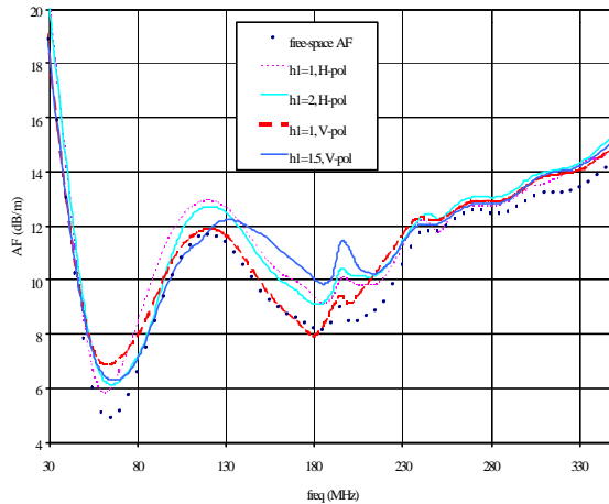
Figure 5. Numerically calculated bicon/log hybrid AF obtained using the 3-m ANSI C63.5 standard site method. The receive antenna is scanned from 1 to 4 m with a step size of 0.05 m. "h1" is transmit height.
